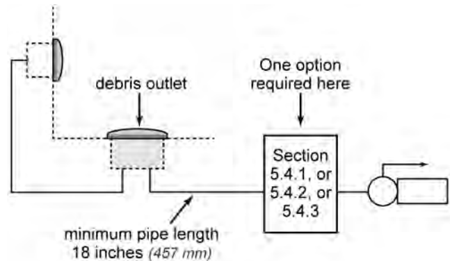
Figure 15. Sumps in series
